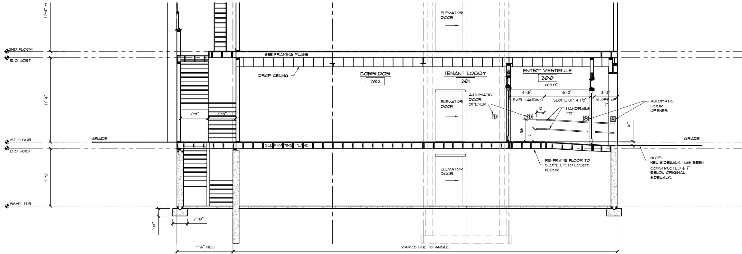
OPTION B BUILDING SECTION ENTRY SIDEWALK RAMP SCALE: \frac{1}{4}''=1'-0''
