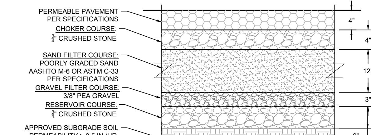
PAVEMENT PATCH NOT TO SCALE
