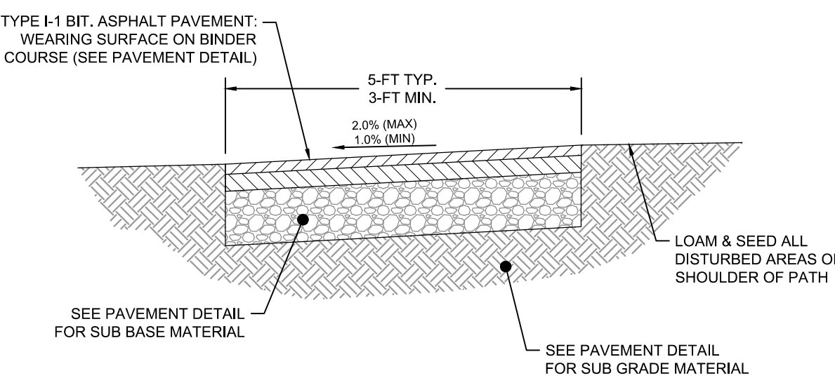
TYPICAL BITUMINOUS PAVEMENT SIDEWALK DETAIL NOT TO SCALE
