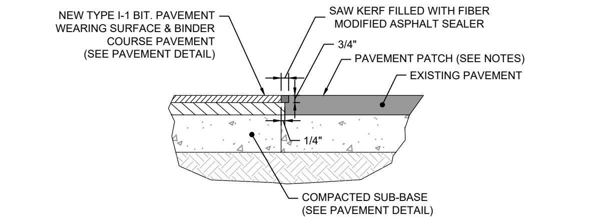
BITUMINOUS PAVEMENT NOT TO SCALE
