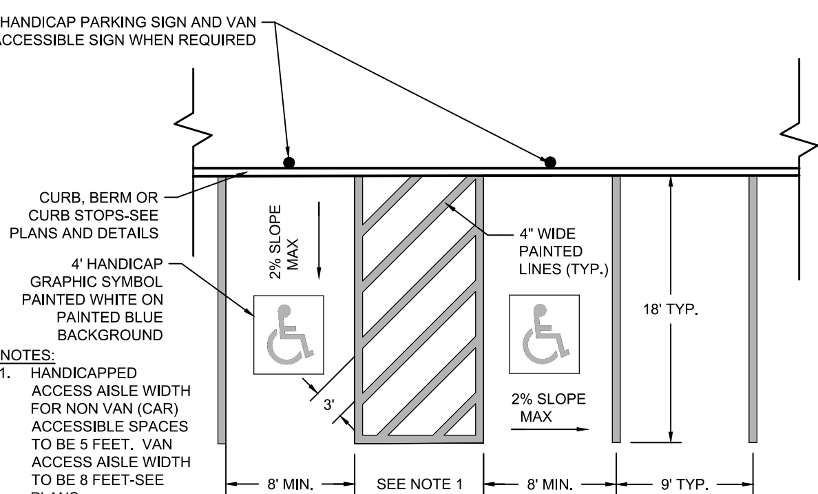
HANDICAPPED AND STANDARD PARKING NOT TO SCALE
