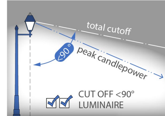
Figure 102. Light fixtures should cut off at maximum of 90 degrees. A cutoff at a lower angle is preferred.
