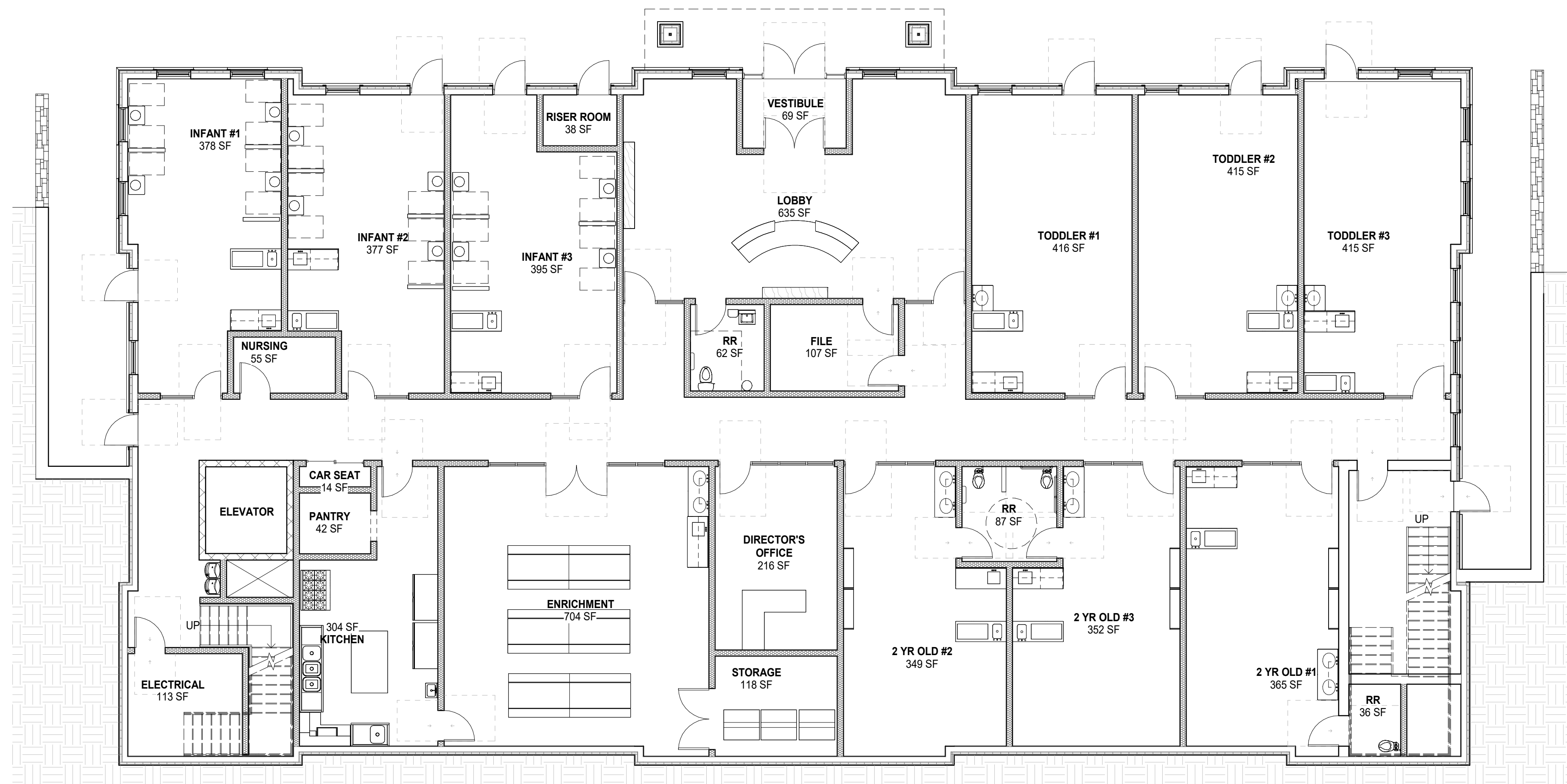
1ST FLOOR
